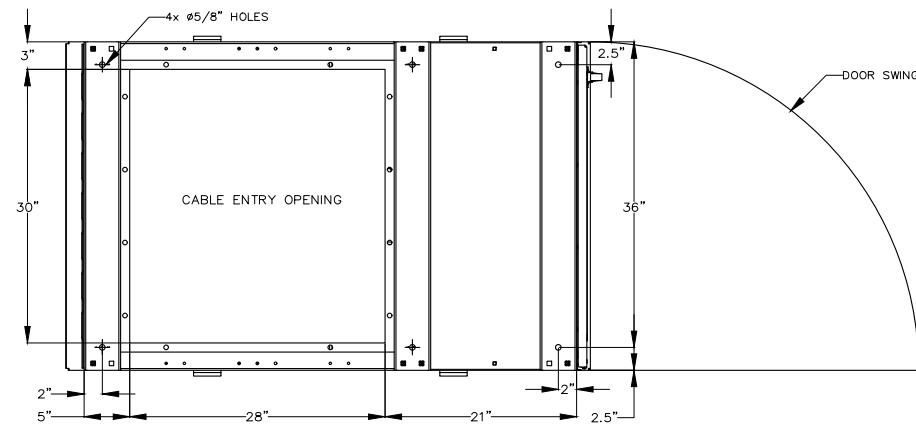
BASE PLAN
