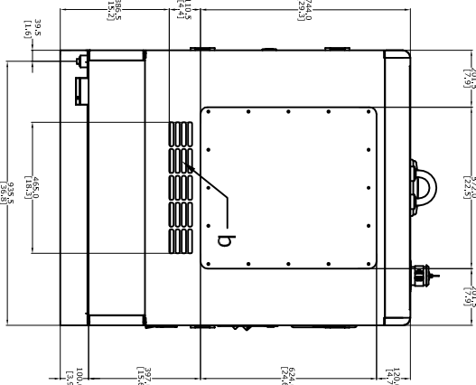
RIGHT VIEW
