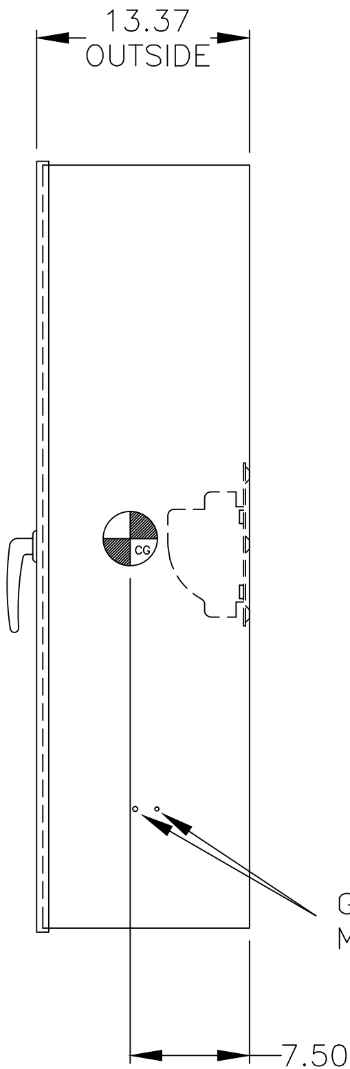
RIGHT SIDE
