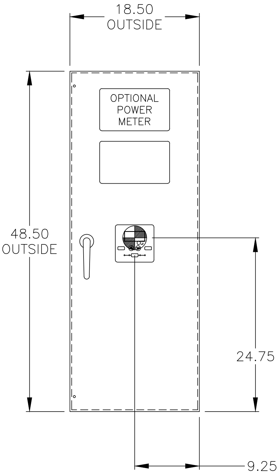
FRONT VIEW WITH DOOR
