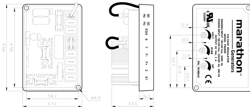
Figure 1 Outline and Drilling Diagram
