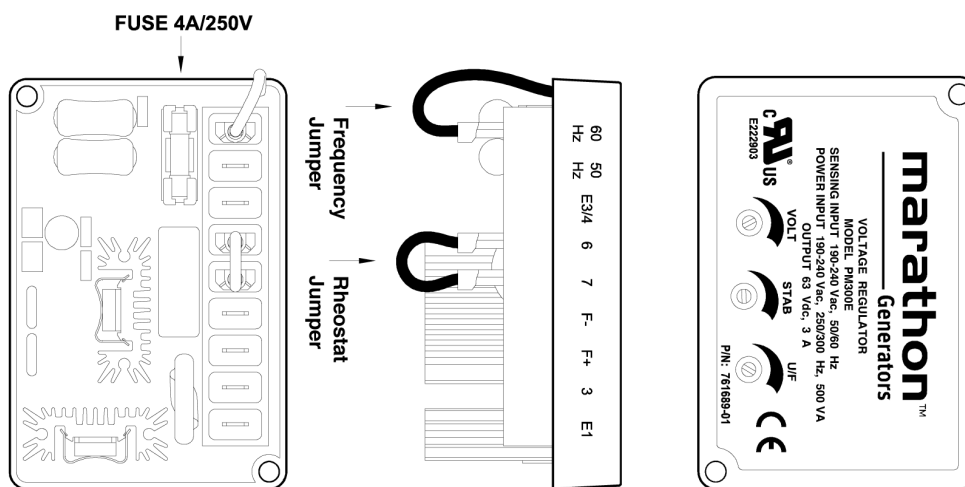
Figure 2 Jumper and Potentiometer Control Locations
