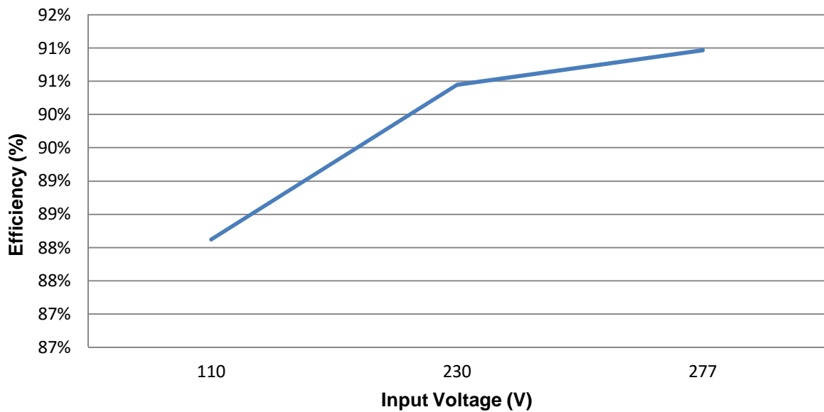
DSE9480 Efficiency Curve at 10 A
