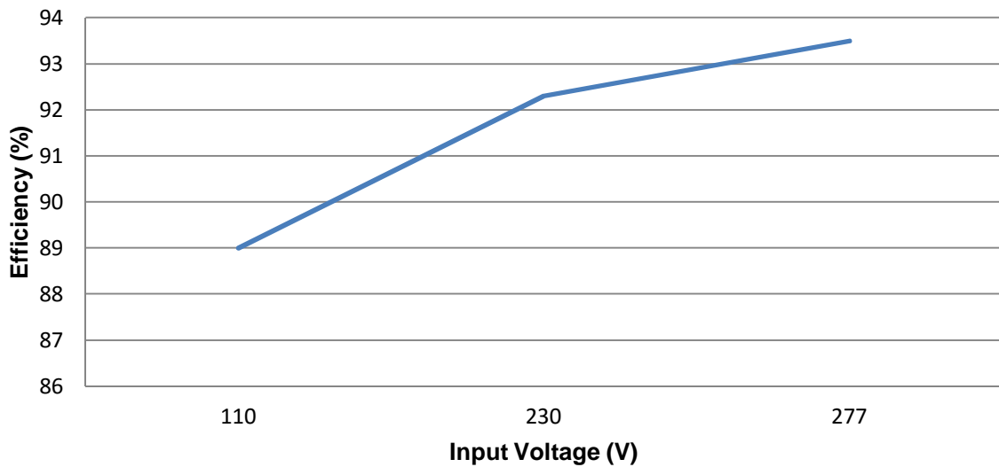
DSE 9473 Efficiency Curve 15 A
