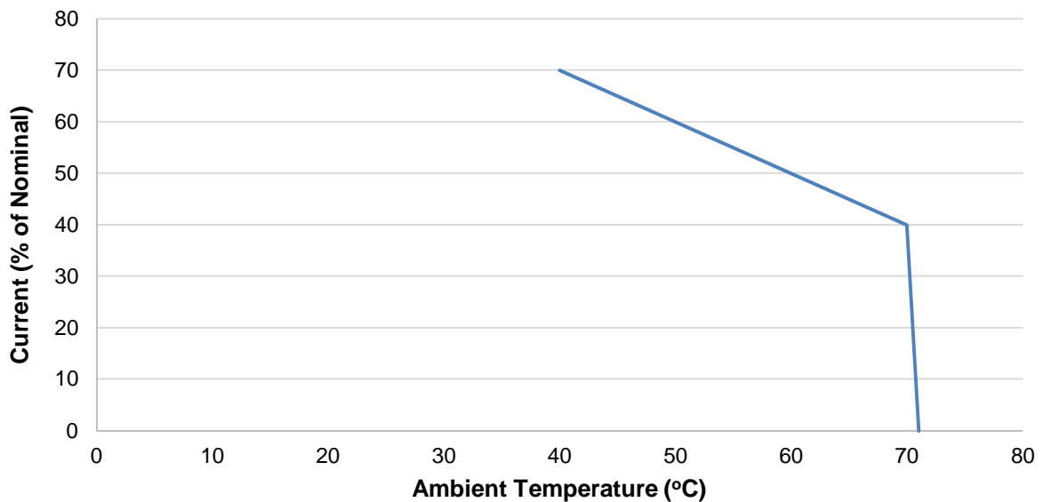
Output Current Derating 90 V < Vin < 110 V and Ambient >= 40 °C
