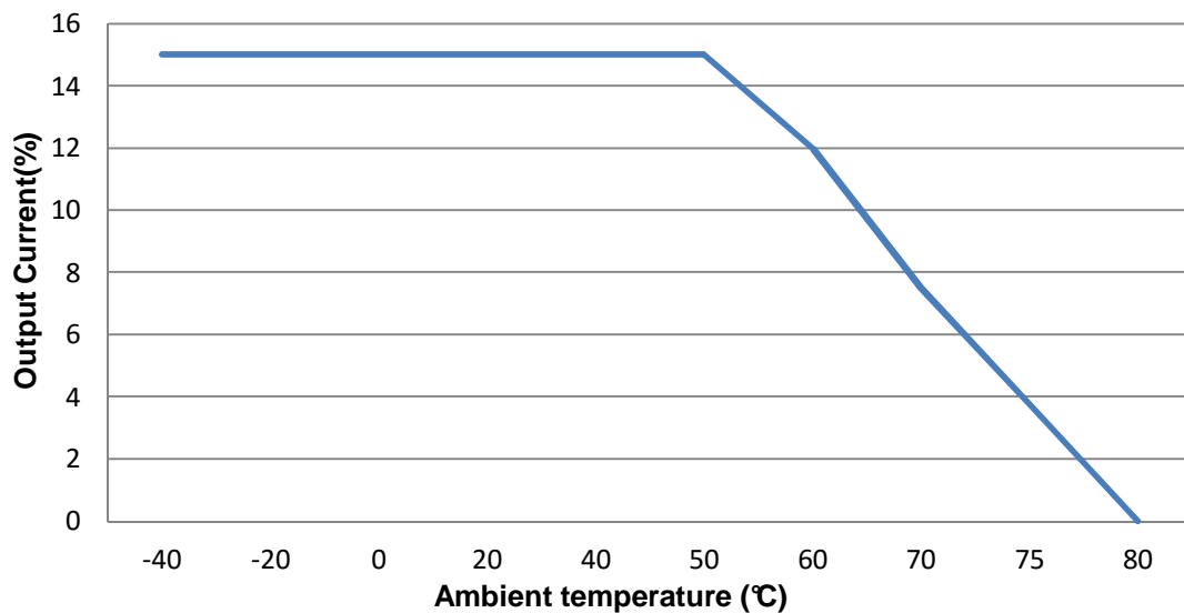
DSE9483 Output Current De-rating Curve 110 V < Vin < 305 V
