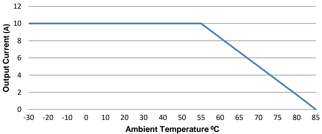
DSE9470 Smart Charger De-rating Curve 110 V < Vin < 305 V
