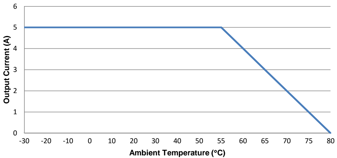
DSE9481 Smart Charger De-rating Curve 90 V < Vin < 305 V
