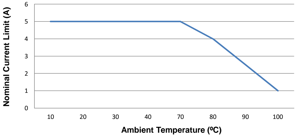
DSE9255 Temperature Derating
