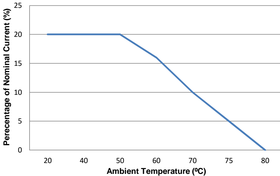
Output Current De-rating Curve 110 V < Vin < 305 V
