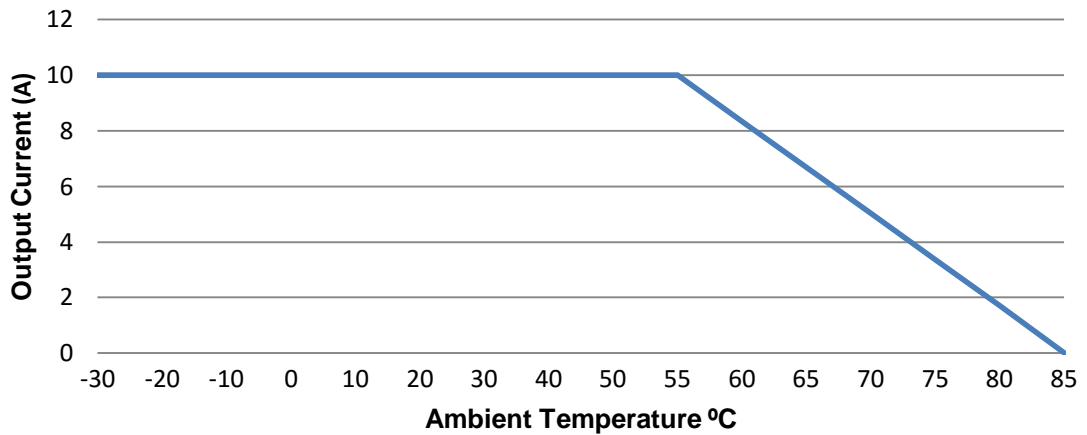
DSE9480 Smart Charger De-rating Curve 110 V < Vin < 305 V
