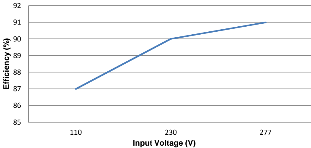
DSE 9483 Efficiency Curve 15 A
