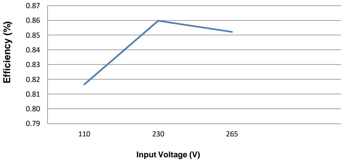
DSE9153 Efficiency Curve at 3 A
