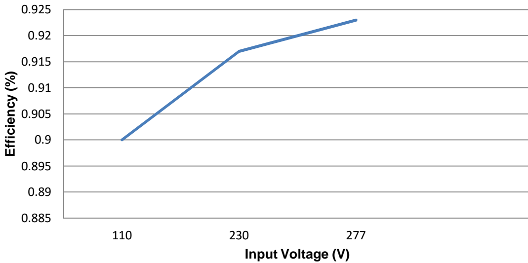
DSE9470 Efficiency Curve at 10 A
