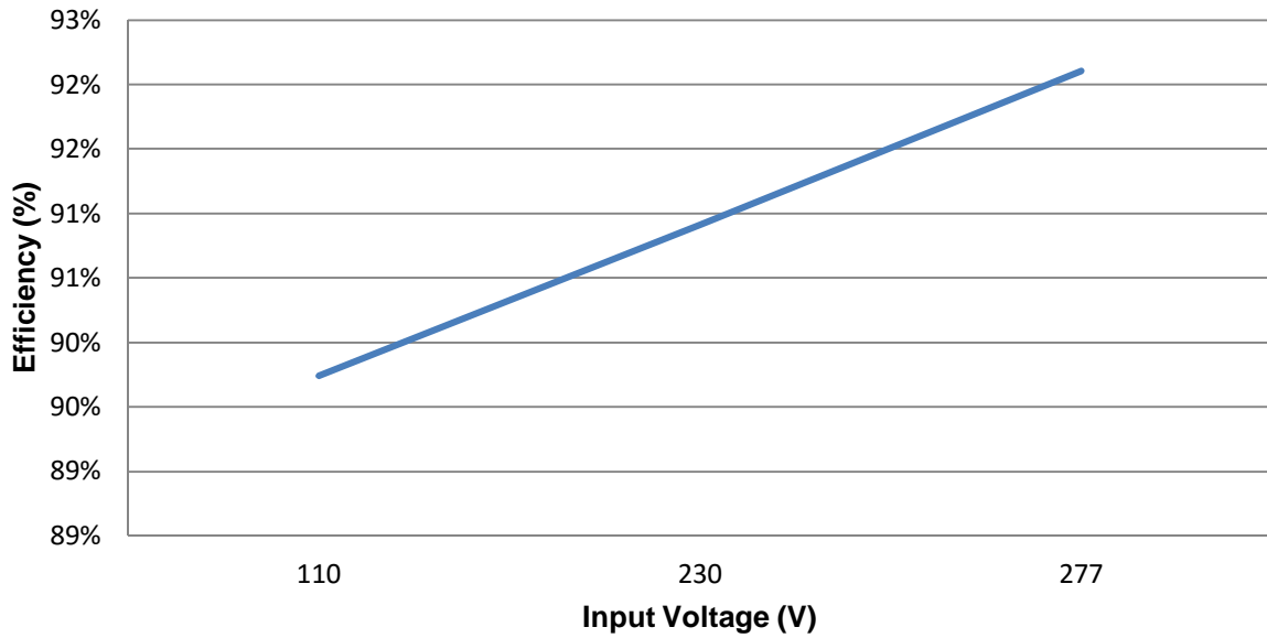
DSE9481 Efficiency Curve at 5 A
