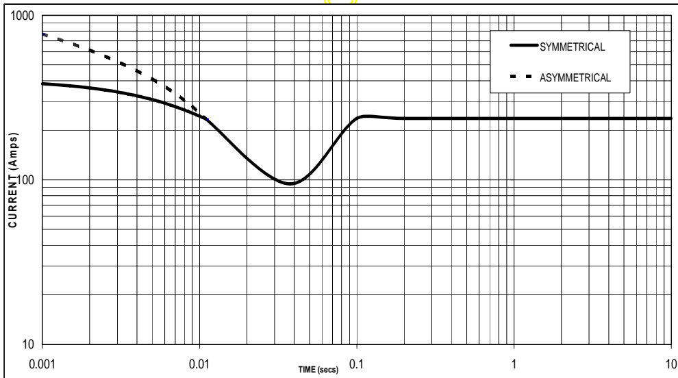
Sustained Short Circuit = 236 Amps
