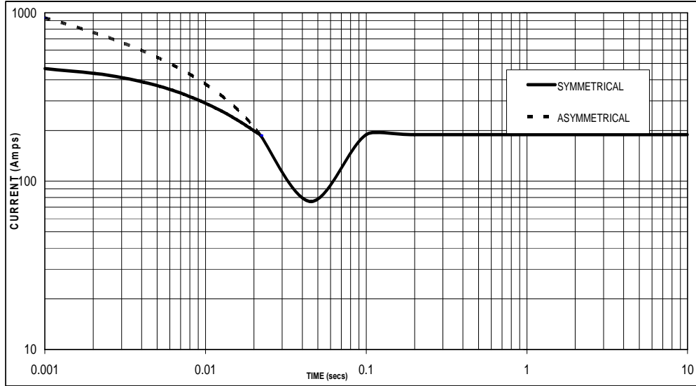
Sustained Short Circuit = 189 Amps
