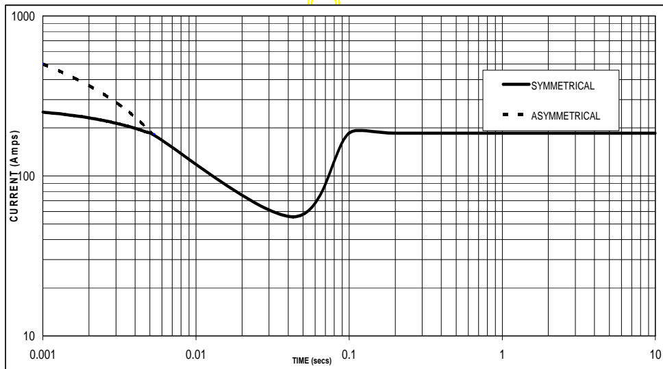
Sustained Short Circuit = 185 Amps
