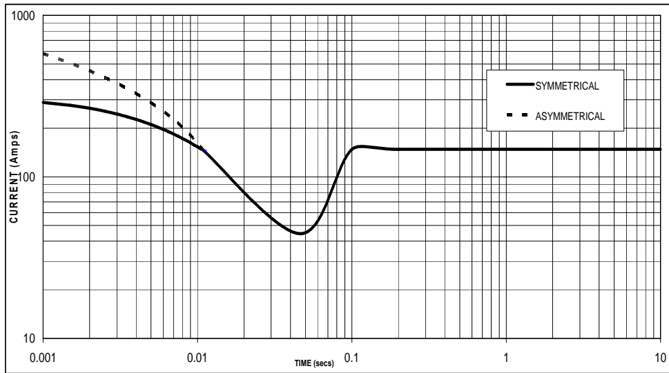
Sustained Short Circuit = 148 Amps
