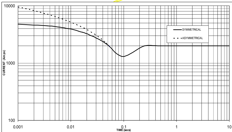
Sustained Short Circuit = 2,000 Amps
