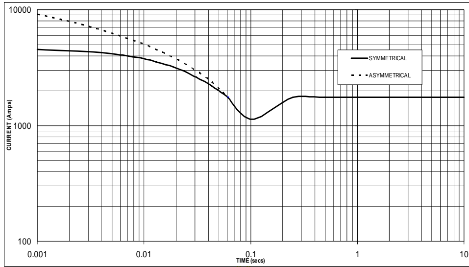
Sustained Short Circuit = 1,750 Amps
