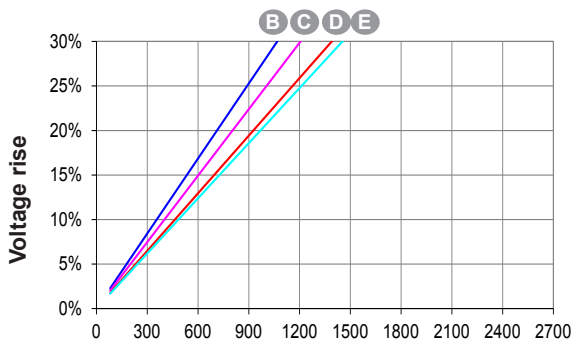
Load shedding (SHUNT) - kVA at P.F. = 0.8
