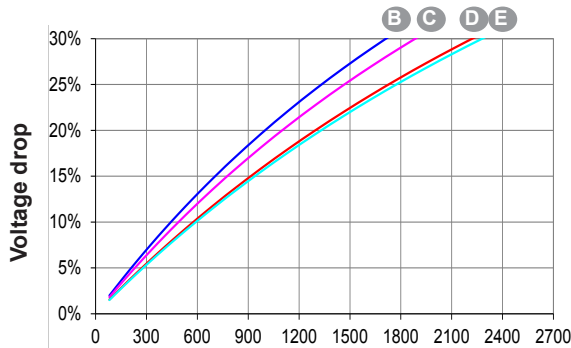
Phase loading (SHUNT) - kVA at P.F. = 0.8
