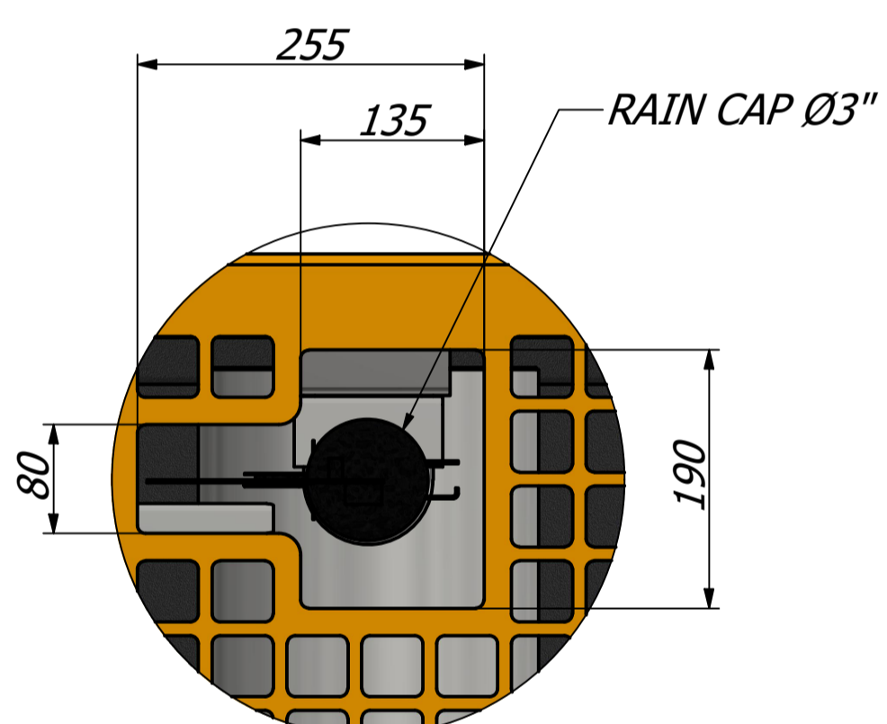
DETAIL B
