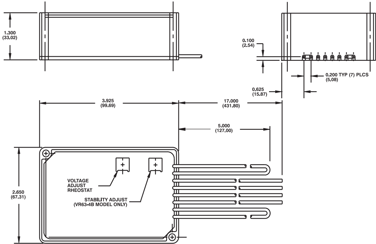
Figure 3 - Outline Drawing
